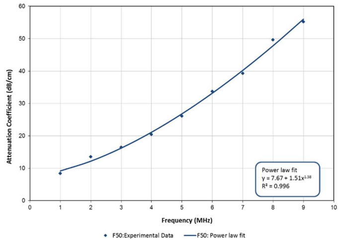
Figure 2 – Attenuation vs Frequency for AptFlex F50
