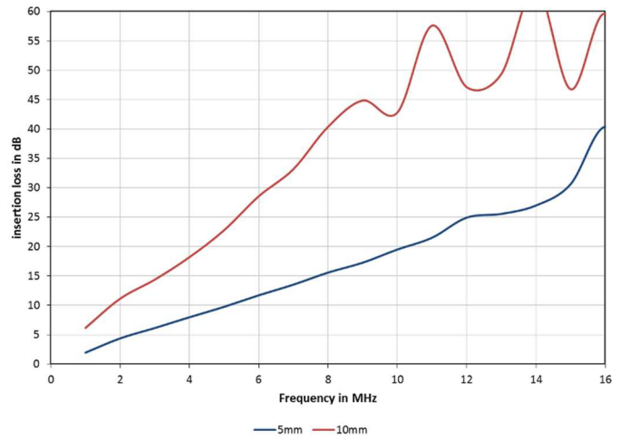
Figure 1 – Insertion loss vs Frequency for AptFlex F50
